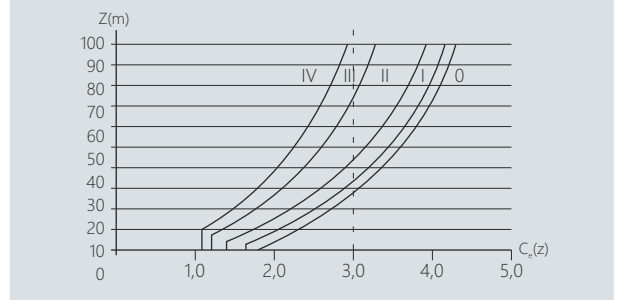
Illustration of the exposure factor C_e(z) for C_0=1.0 , k_1=1.0
